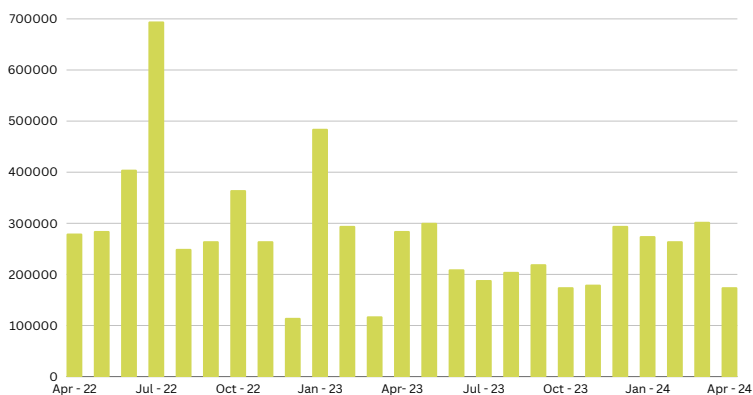
Nonfarm payroll employment, over-the-month change, seasonally adjusted, April 2022 - April 2024
